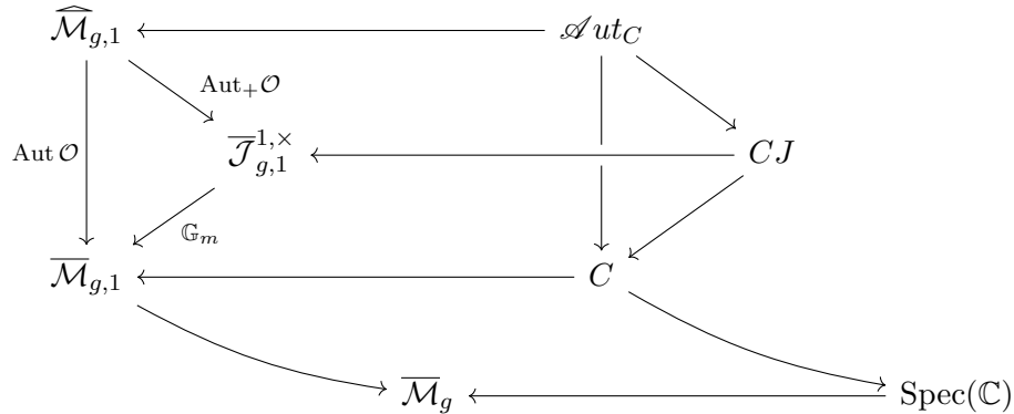
FIGURE 2. The definition of \mathcal{A}ut_C and CJ . The curve C is identified with the fiber of \overline{\mathcal{M}}_{g,1} \rightarrow \overline{\mathcal{M}}_g over the moduli point [C] \in \overline{\mathcal{M}}_g .
