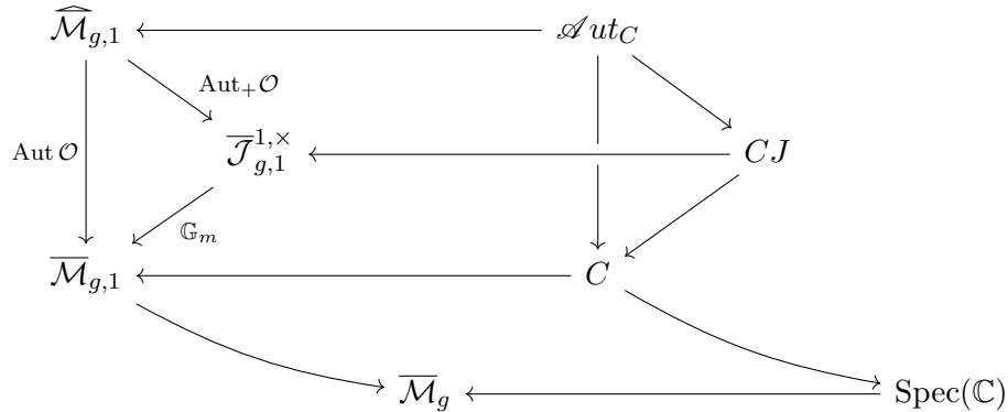
FIGURE 2. The definition of \mathcal{A}ut_C and CJ .
